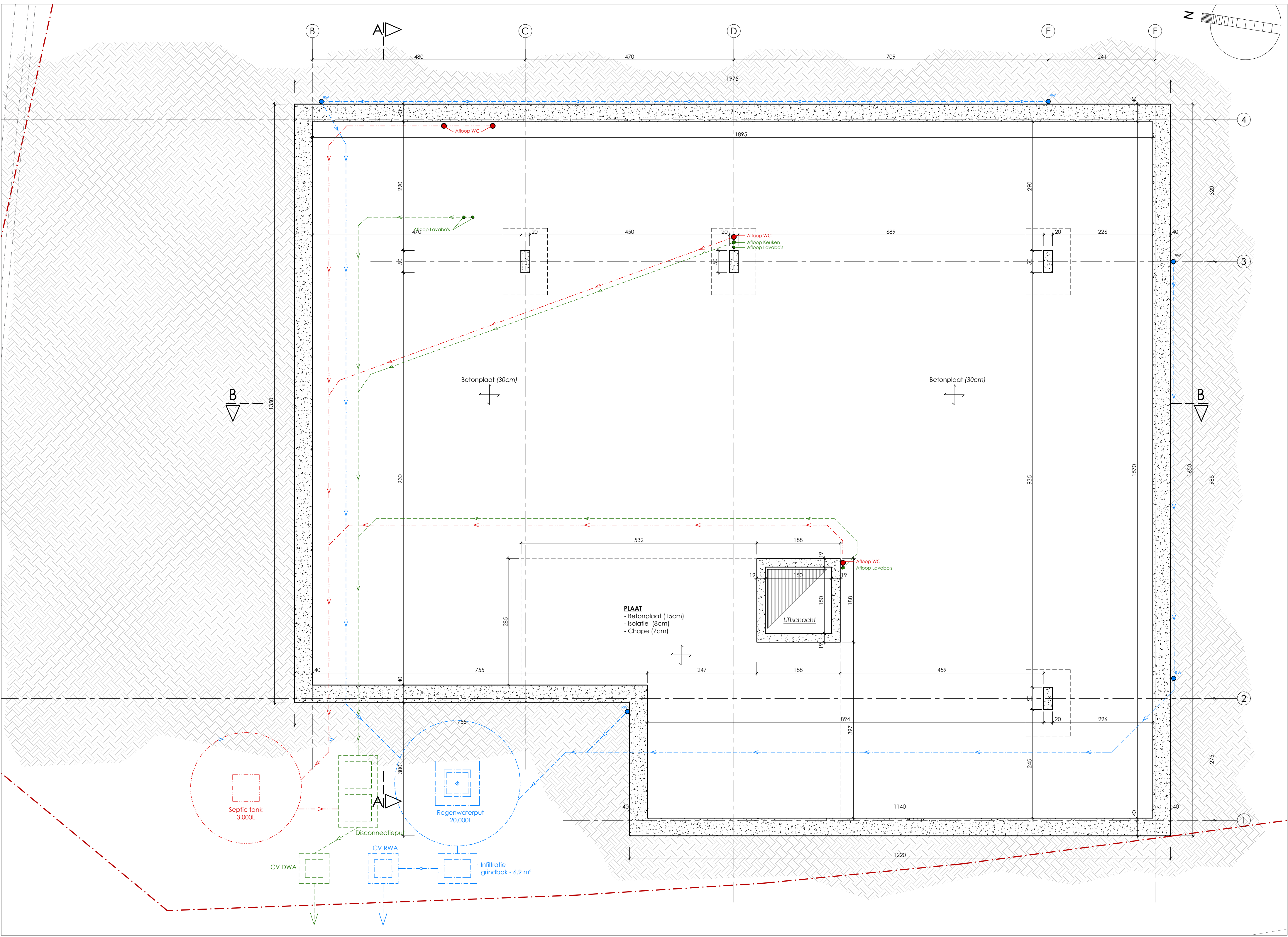
Funderingsplan - 1/50
