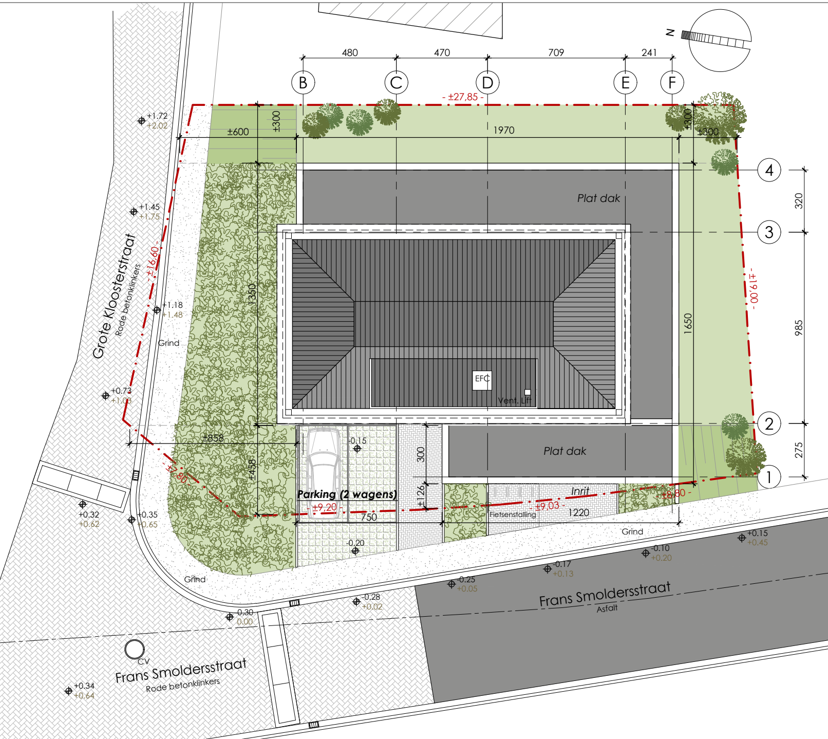
Inplantingsplan - 1/200
