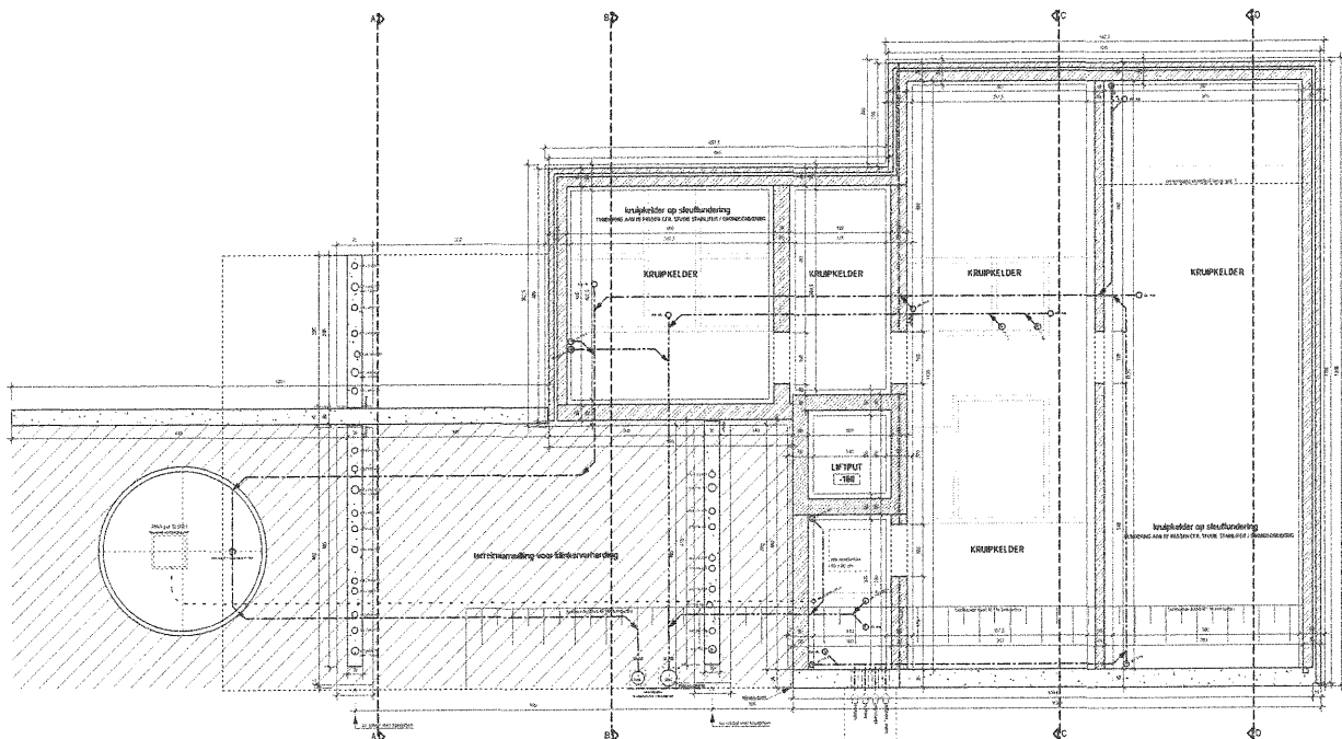
FUNDERINGS- & RIOLERINGSPLAN
